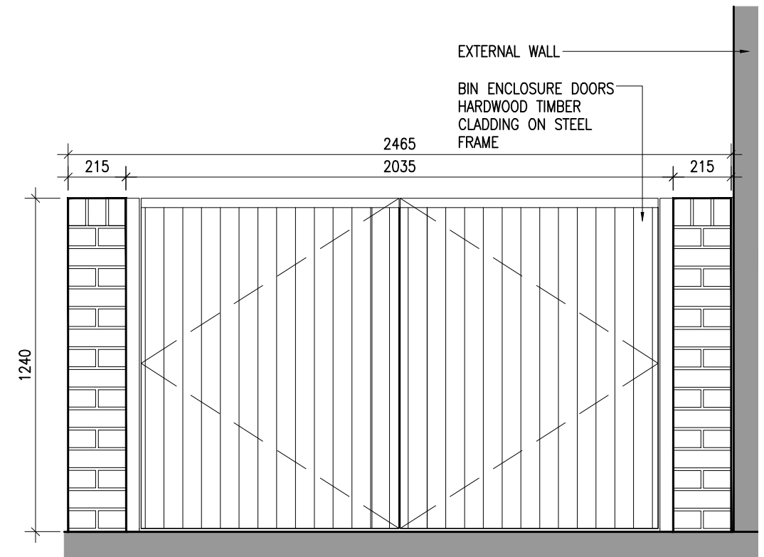
03 Front Elevation 1:50@A3
